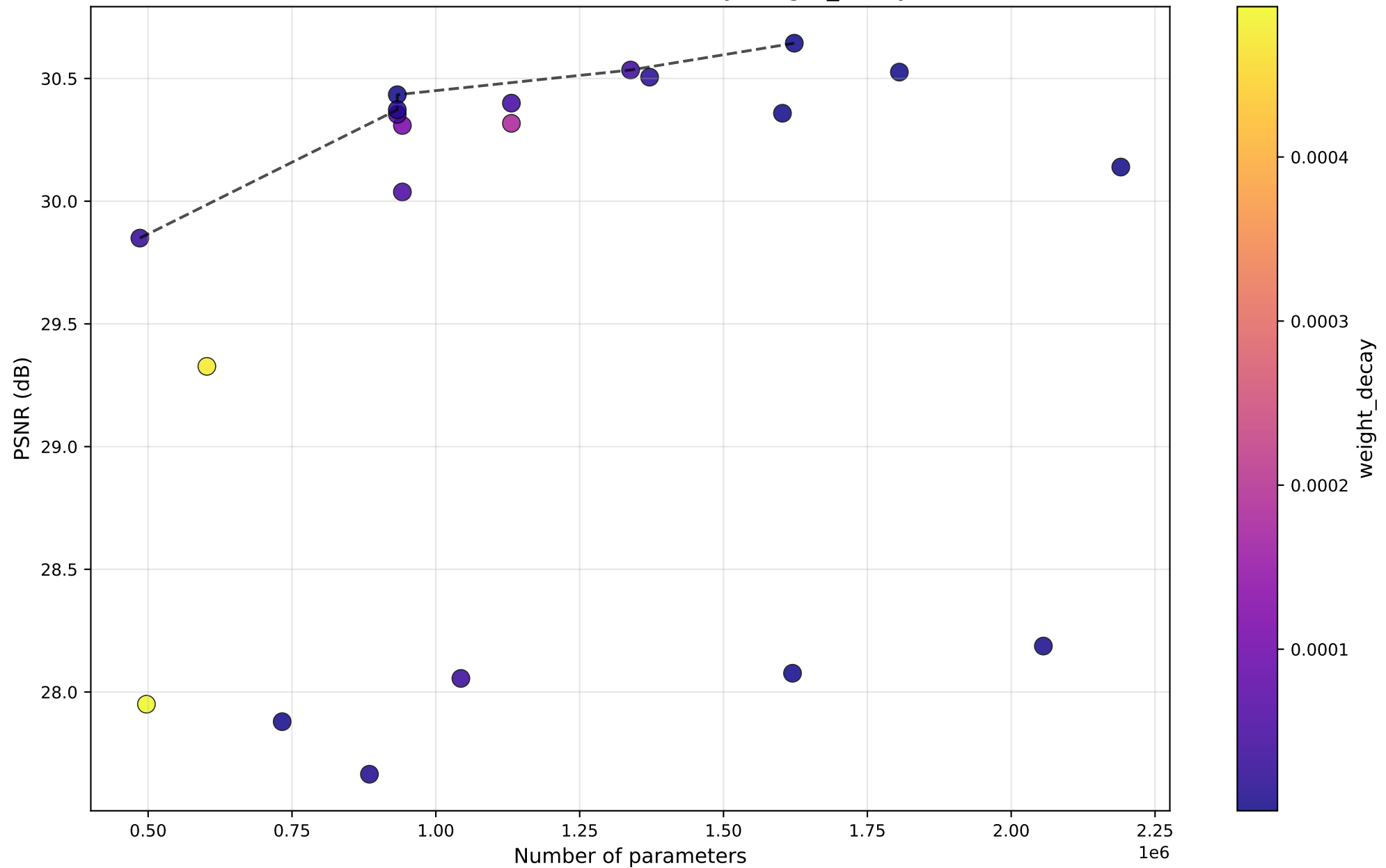
PSNR vs #Params — ELAN — by weight_decay
